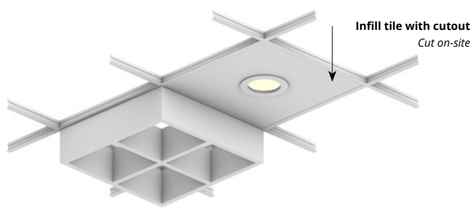
Recessed light
