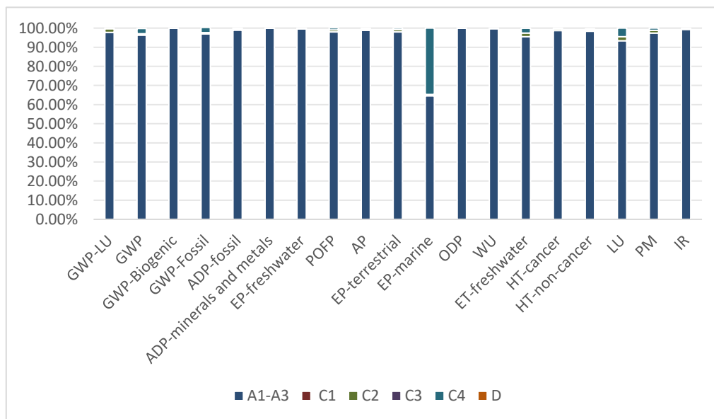
Figure 4. Printed Panel each stage contribution to LCA results
