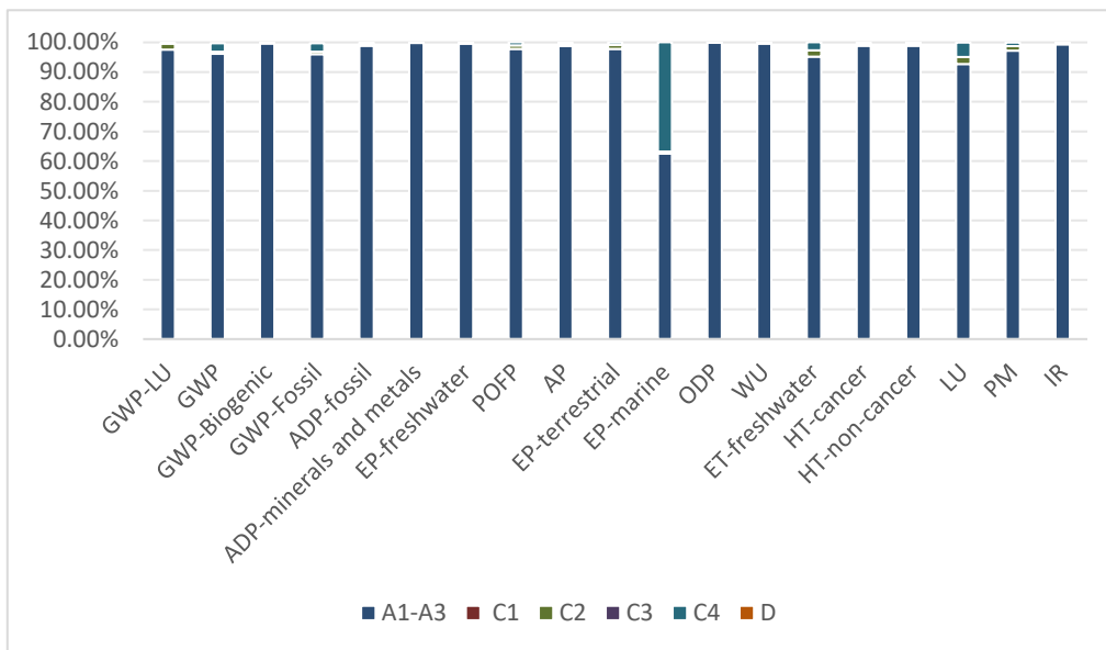
Figure 4. Creative Cut Screens each stage contribution to LCA results
