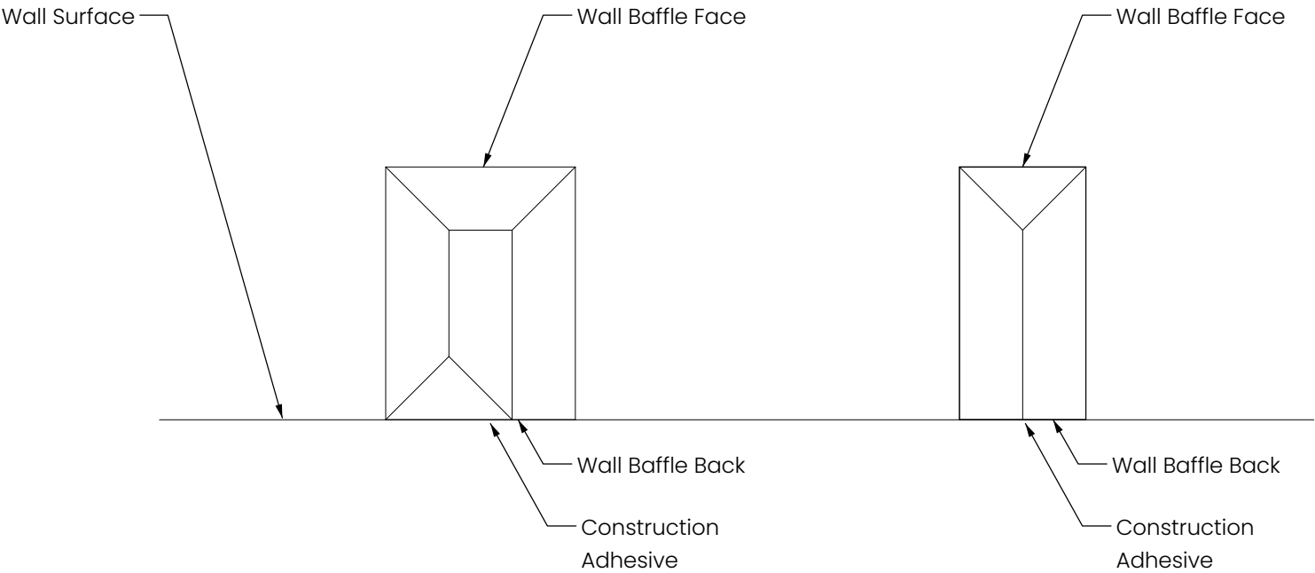
Installation Detail NTS, For representation only 01
