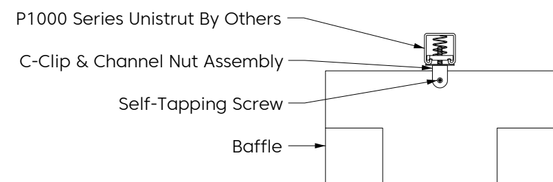
Threaded Rod To Unistrut
