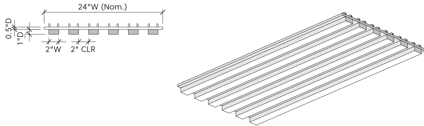
Linear Narrow Plank 2"W x 1"D Slat Profile
